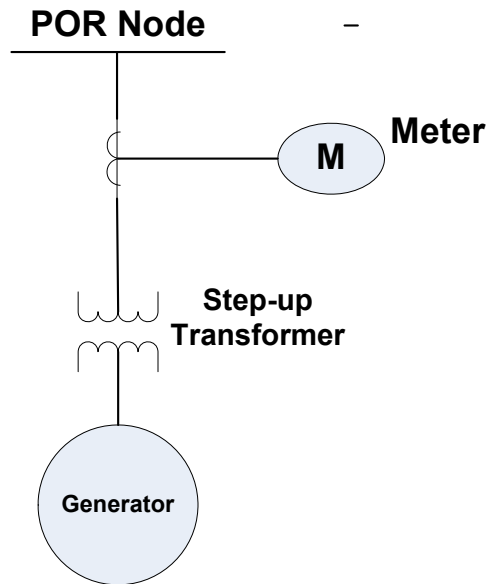
Exhibit 4-5: Generating Unit with POR at Station
