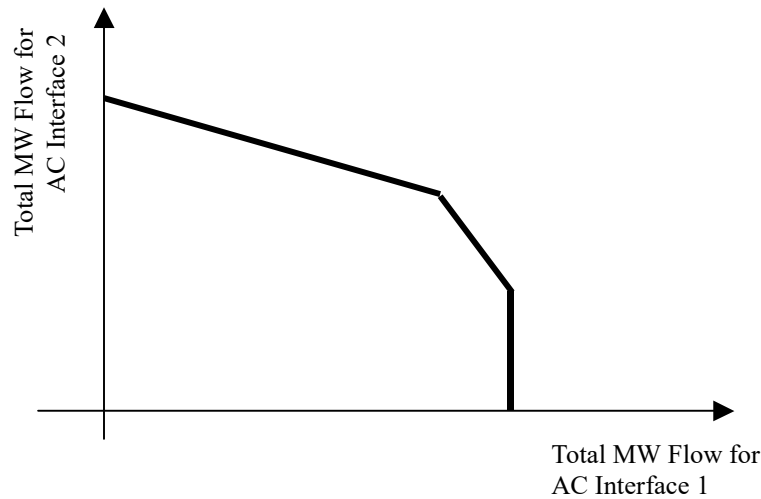
Exhibit 4-13: AC Interface MW Flow vs. Interface MW Flow Constraint
